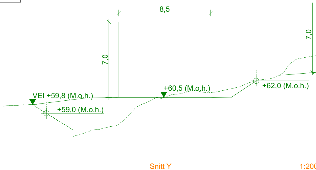
SNITT Y-Y
