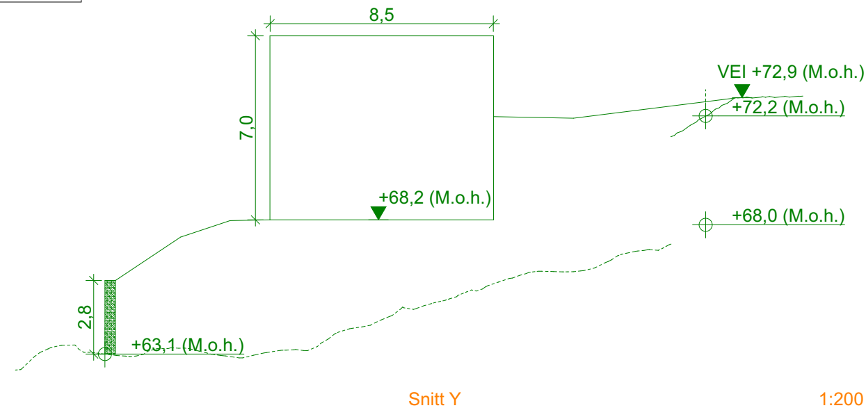
SNITT Y-Y
